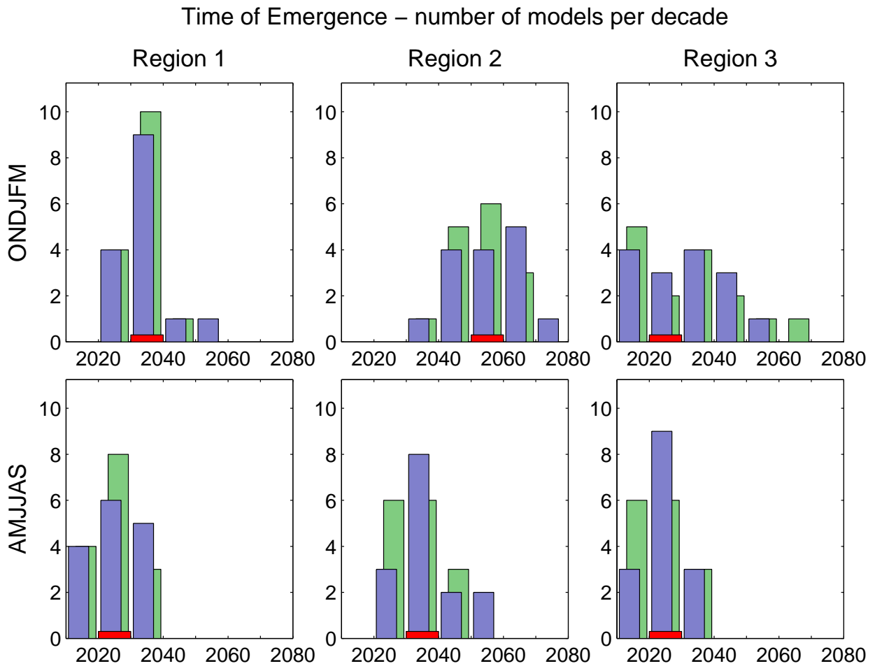
Figure S3: Time of emergence for surface air temperatures for three equal area regions as indicated in Fig. 4. October-March (top) and April-September (bottom). Histograms representing the number of models of when the first year temperature has expected S/N > 2 , using each GCM's own variability (blue) and median signal (green).
