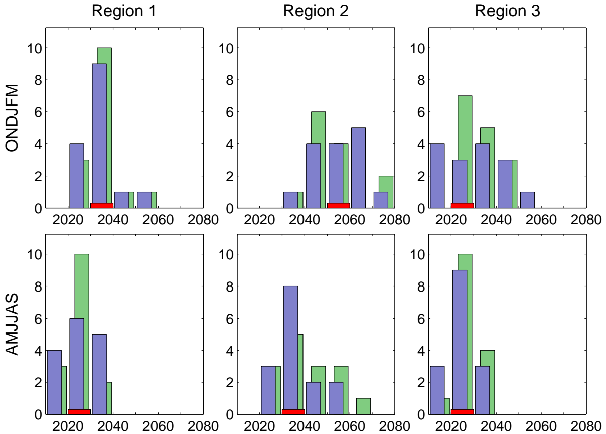
Figure 4. Time of emergence for surface air temperatures for three equal area regions as indicated in Fig. 3. October-March (top) and April-September (bottom). Histograms representing the number of models which cross the S/N > 2 temperature threshold in each decade, using each GCM’s own variability (blue) and median variability (green). The red bars indicate the decade of ToE when using both the median signal and median noise.
