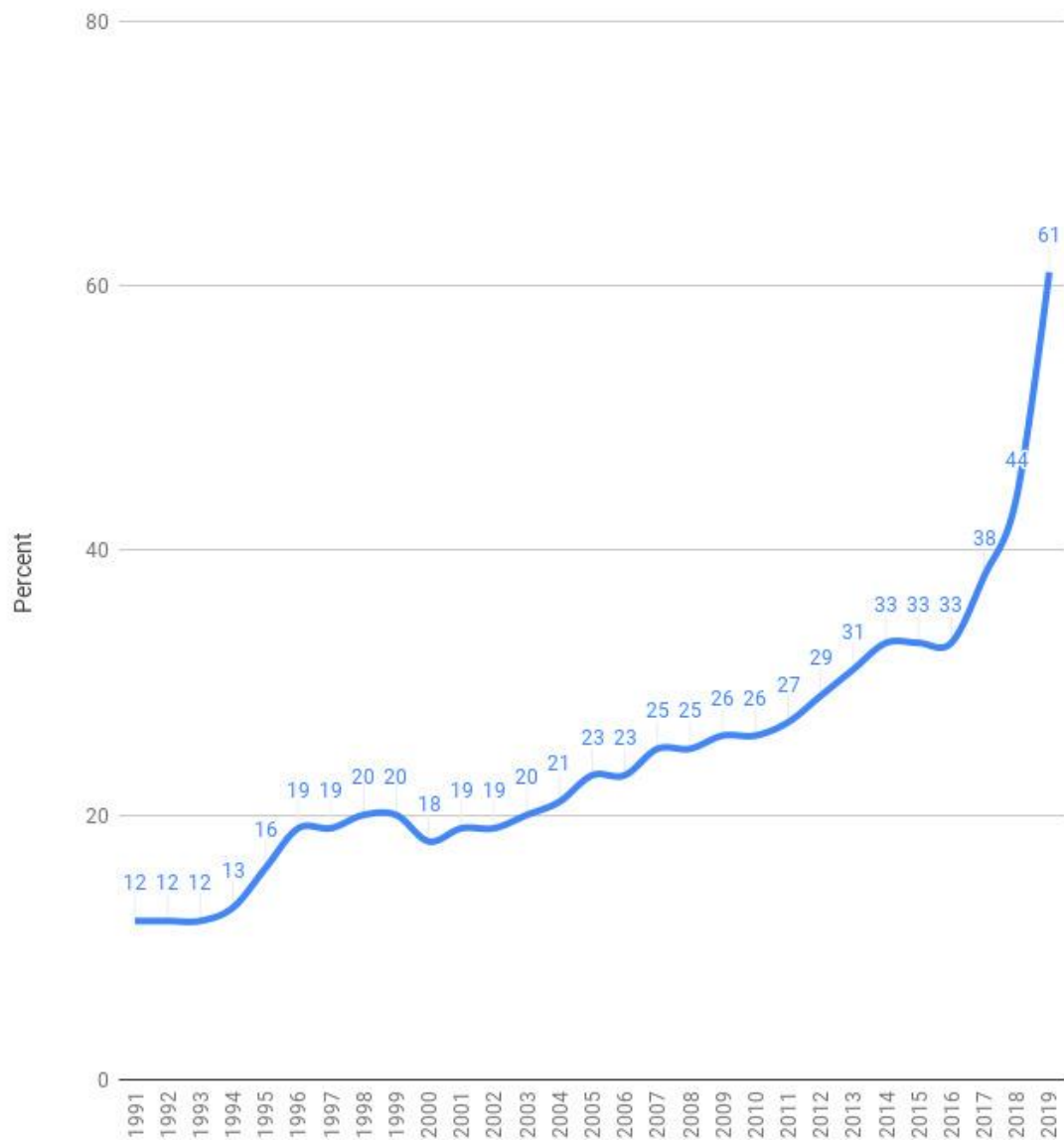
Percent Of USHCN Monthly Temperature Data Which Is Fabricated
