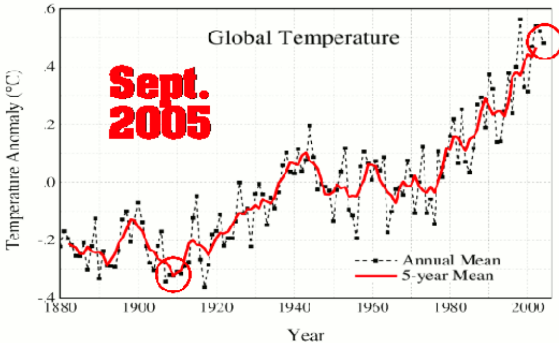
NASA Global Land-Ocean Temperature 'Adjustments'
