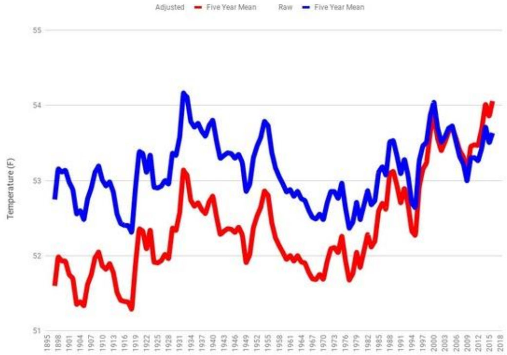
Average Monthly Temperature At All US Historical Climatology Network Stations
