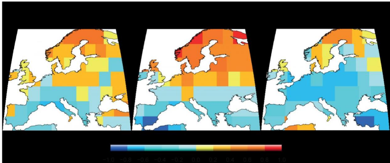
IMAGE: THESE ARE MAPS SHOWING DECADAL CORRELATION DURING THE 20TH CENTURY BETWEEN INSTRUMENTAL MEASUREMENTS OF TEMPERATURE AND PRECIPITATION (LEFT), TREE-RING RECONSTRUCTED TEMPERATURE AND DROUGHT (MIDDLE), AND MODEL-SIMULATED TEMPERATURE AND PRECIPITATION (RIGHT)... viewmore
